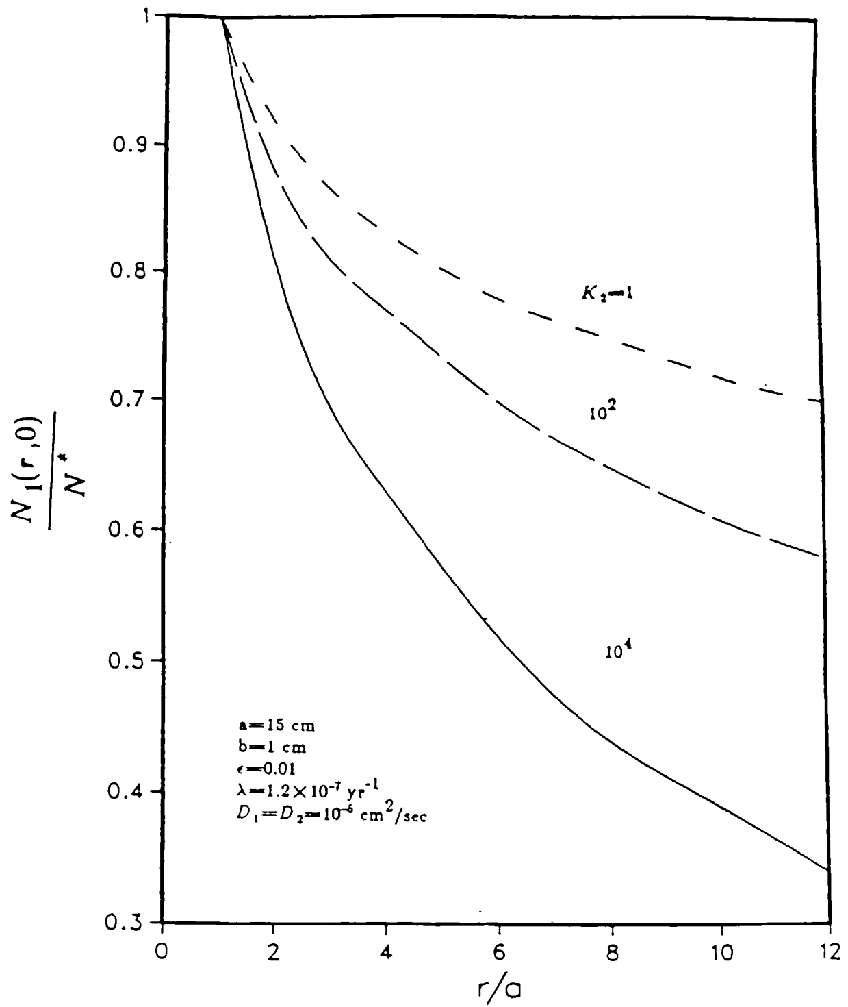
Figure 3 Variation of normalized concentration with r/a for different retardation coefficients.
